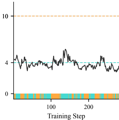
Client 5 (float16/int8)
