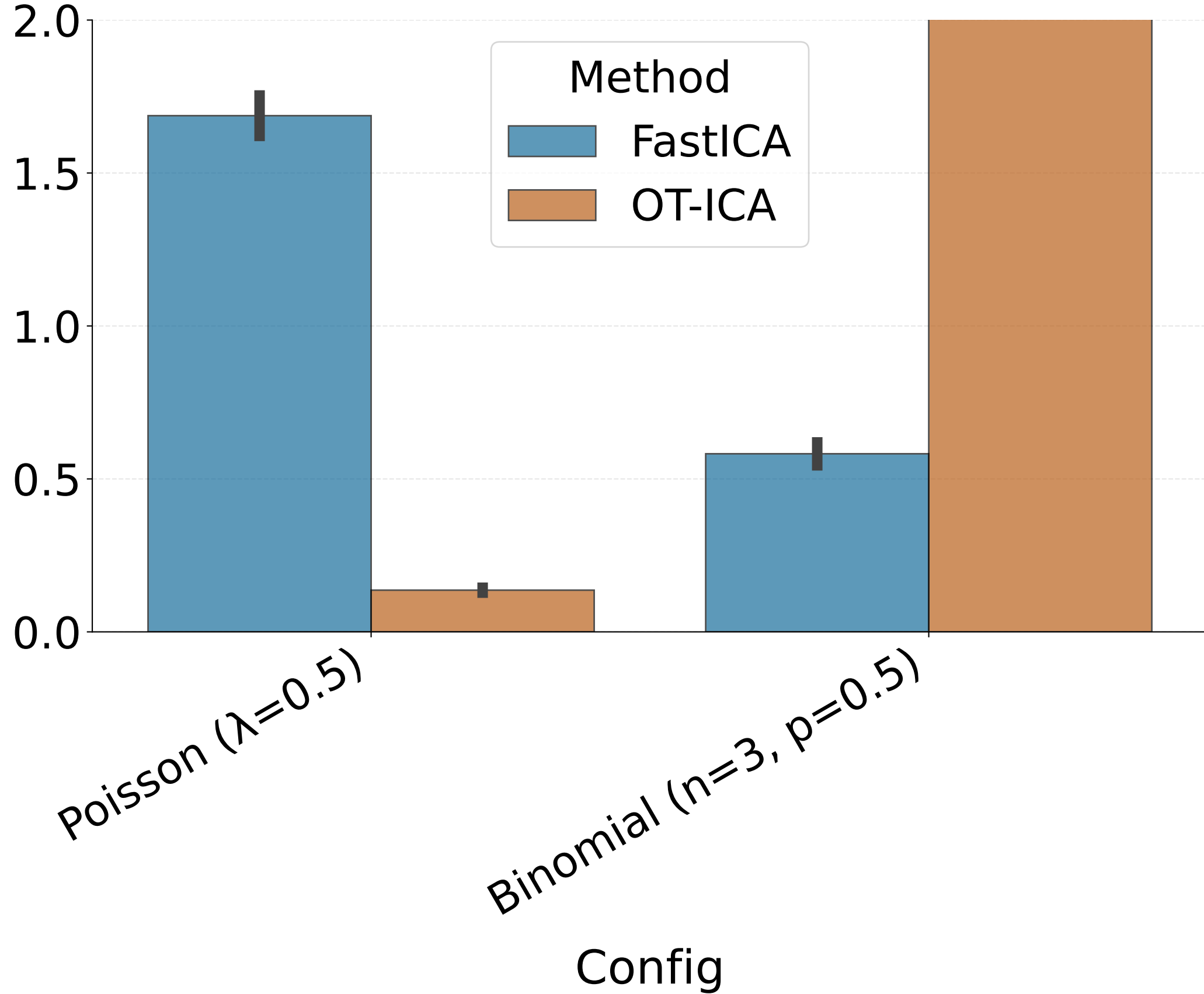
Amari Error: Highly Non-Gaussian Discrete
