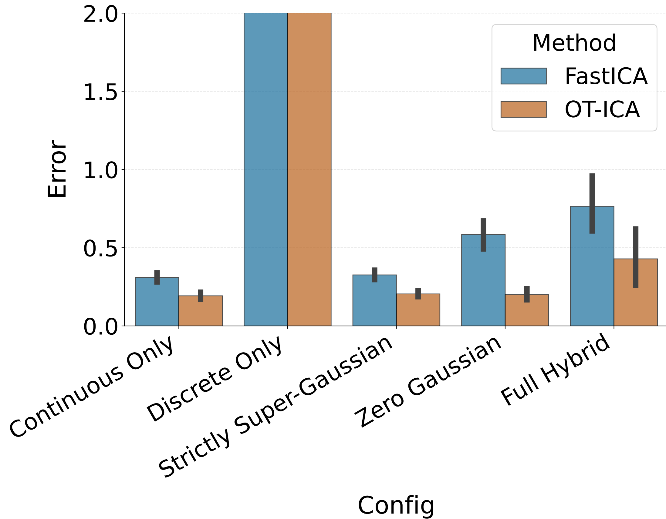
Amari Error: Sub-Pool Ablation
