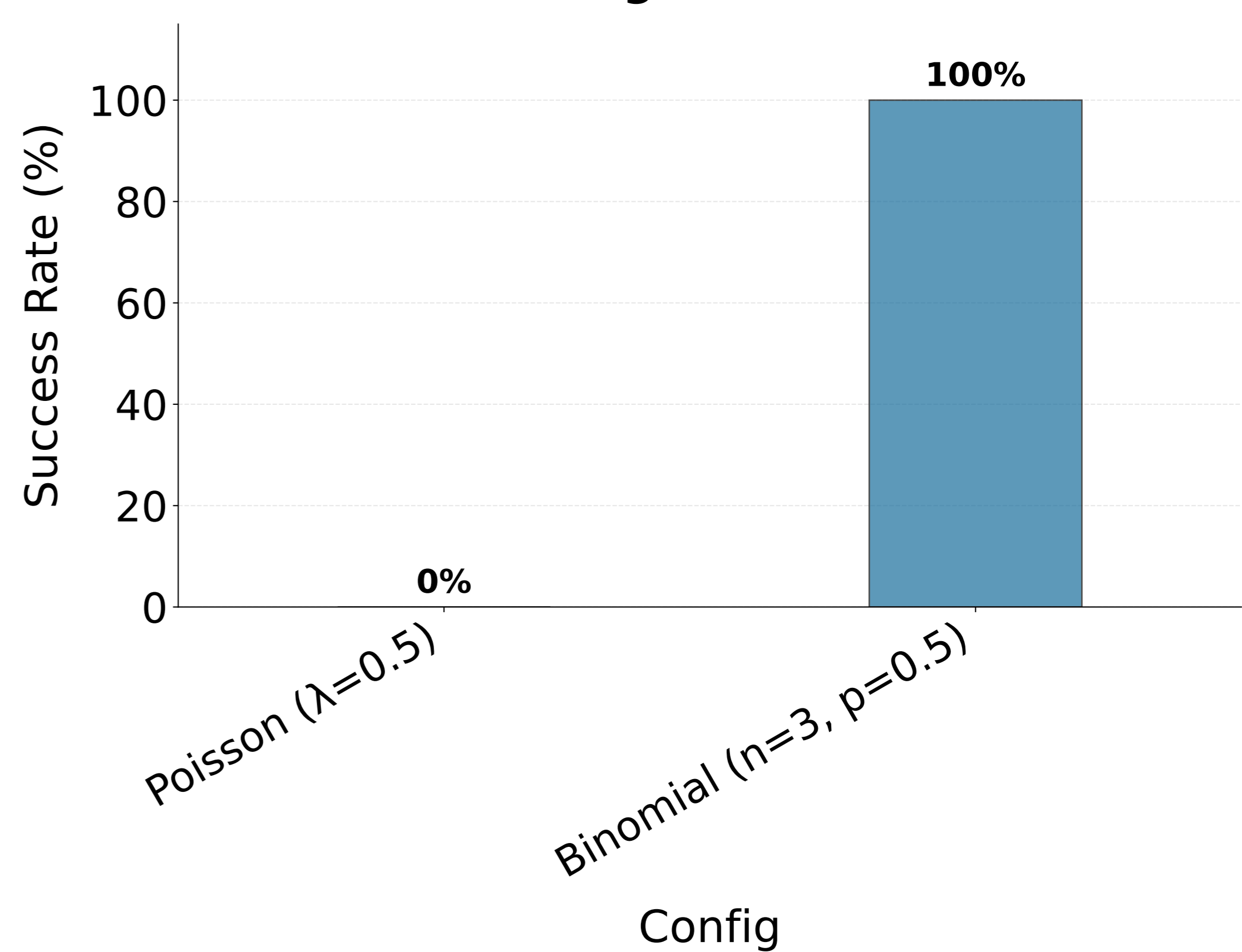
FastICA Convergence: Harsh Discrete
