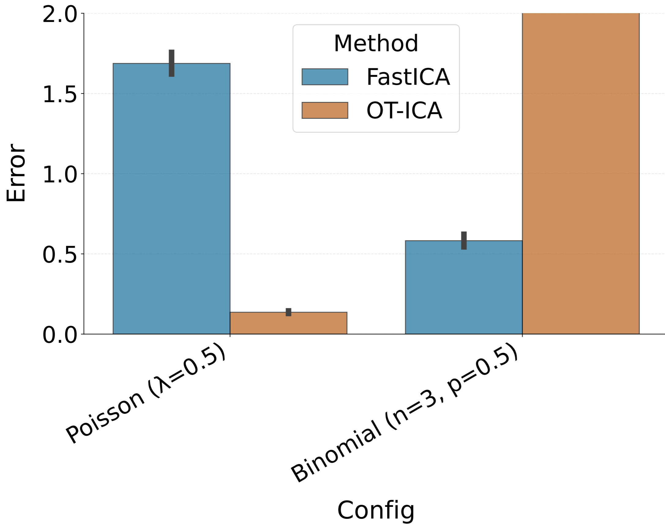
Amari Error: Harsh Discrete
