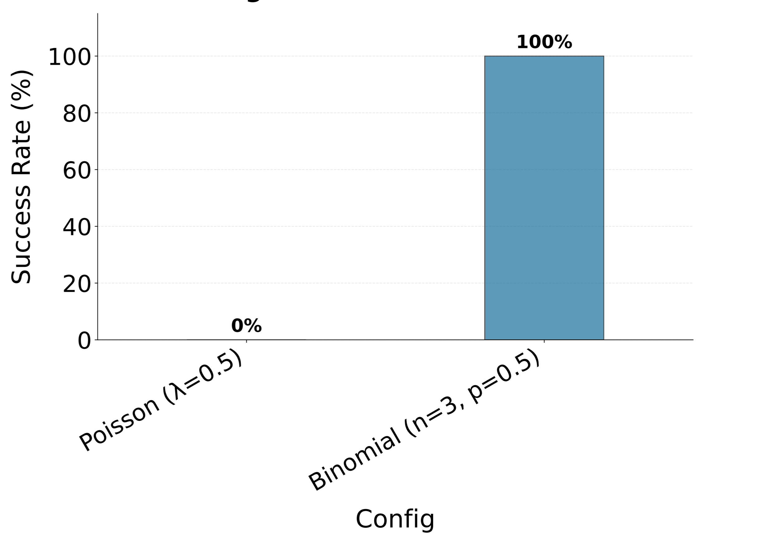
FastICA Convergence: Harsh Discrete Environments
