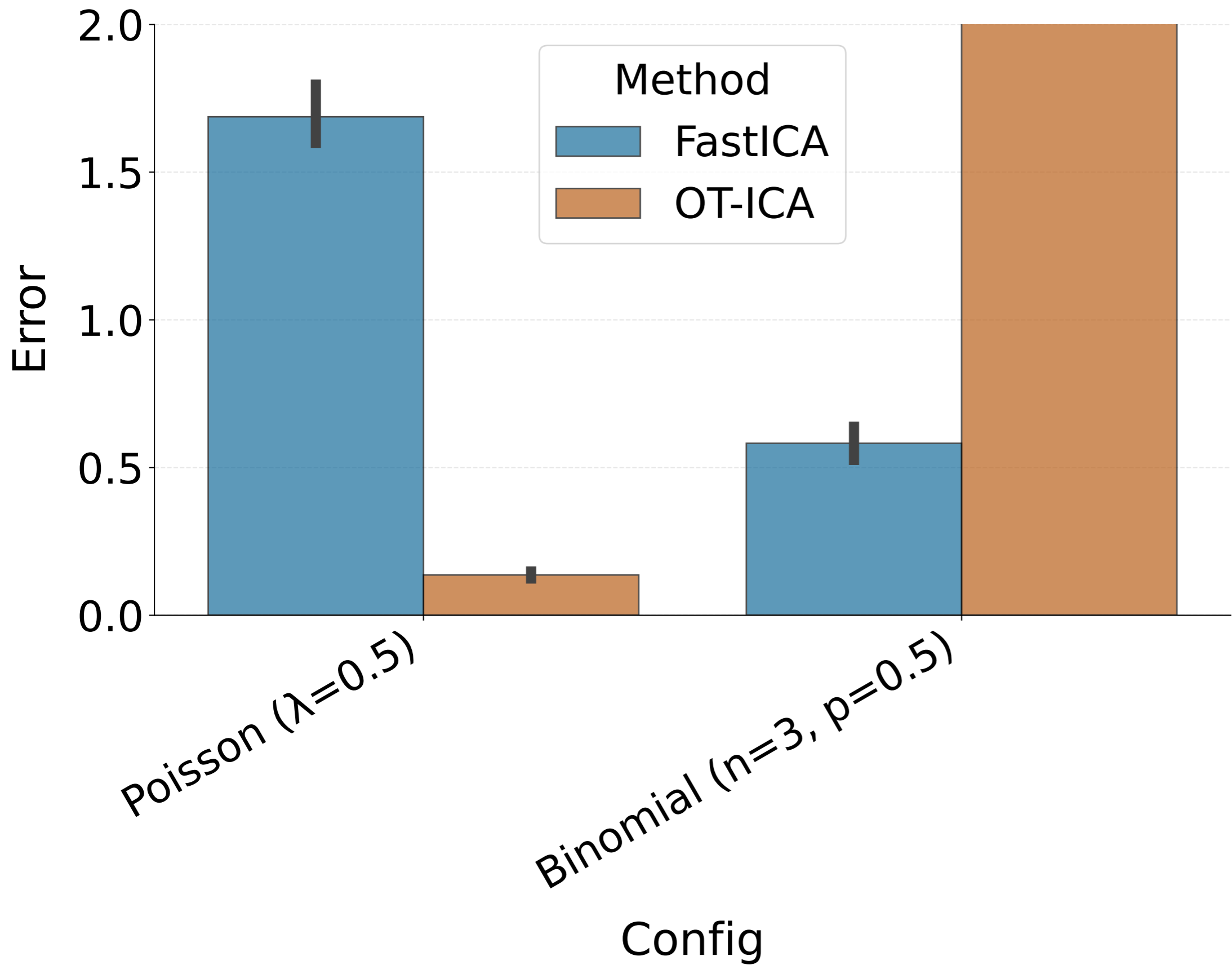
Amari Error: Harsh Discrete Environments
