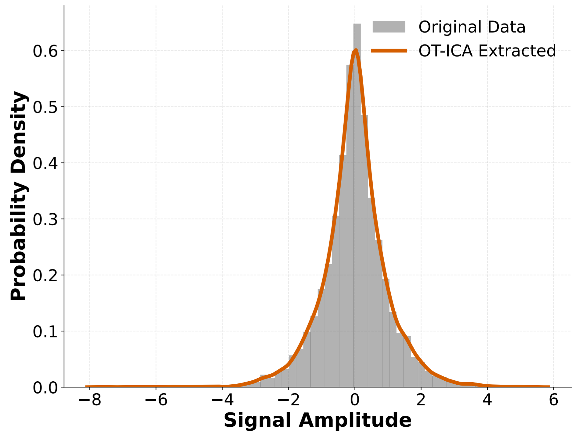
Component 4: Recovered Laplace
