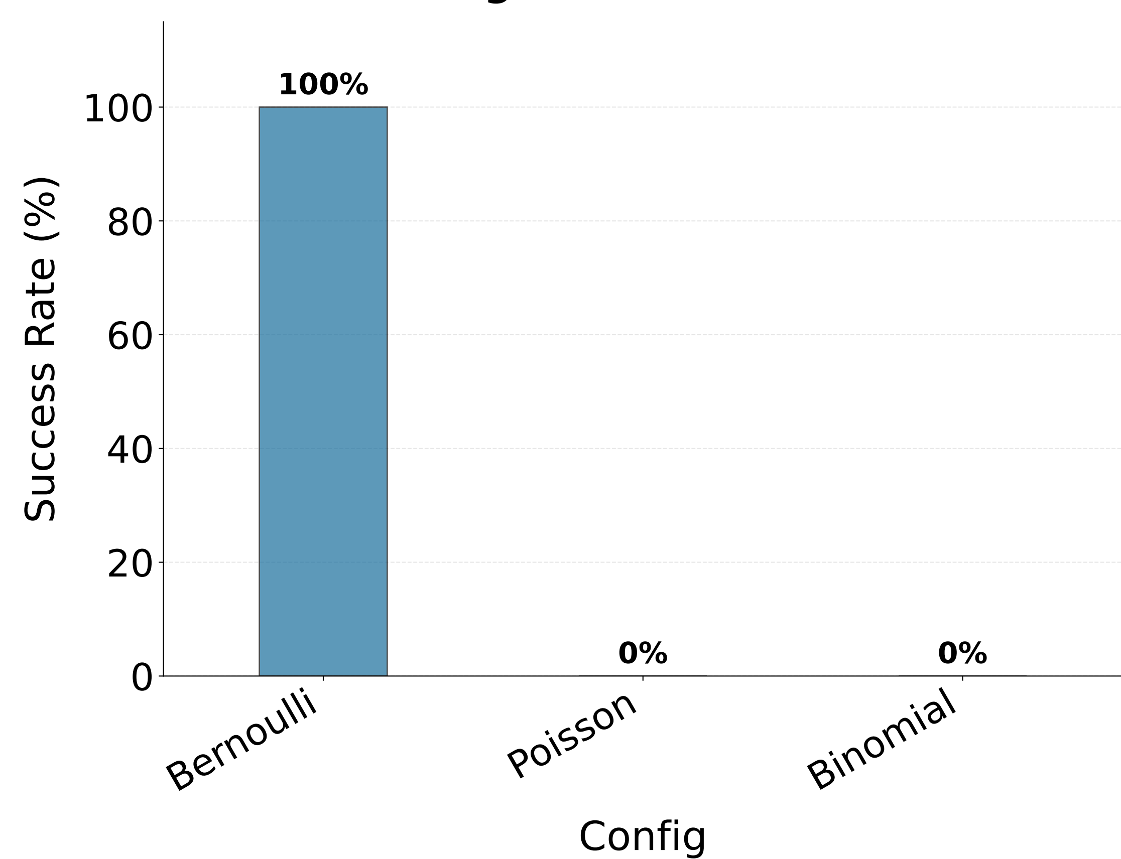
FastICA Convergence: Discrete Distributions
