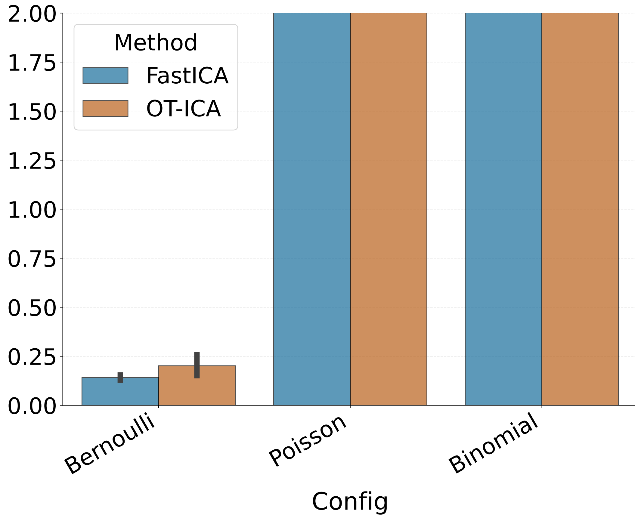
Amari Error: Discrete Distributions
