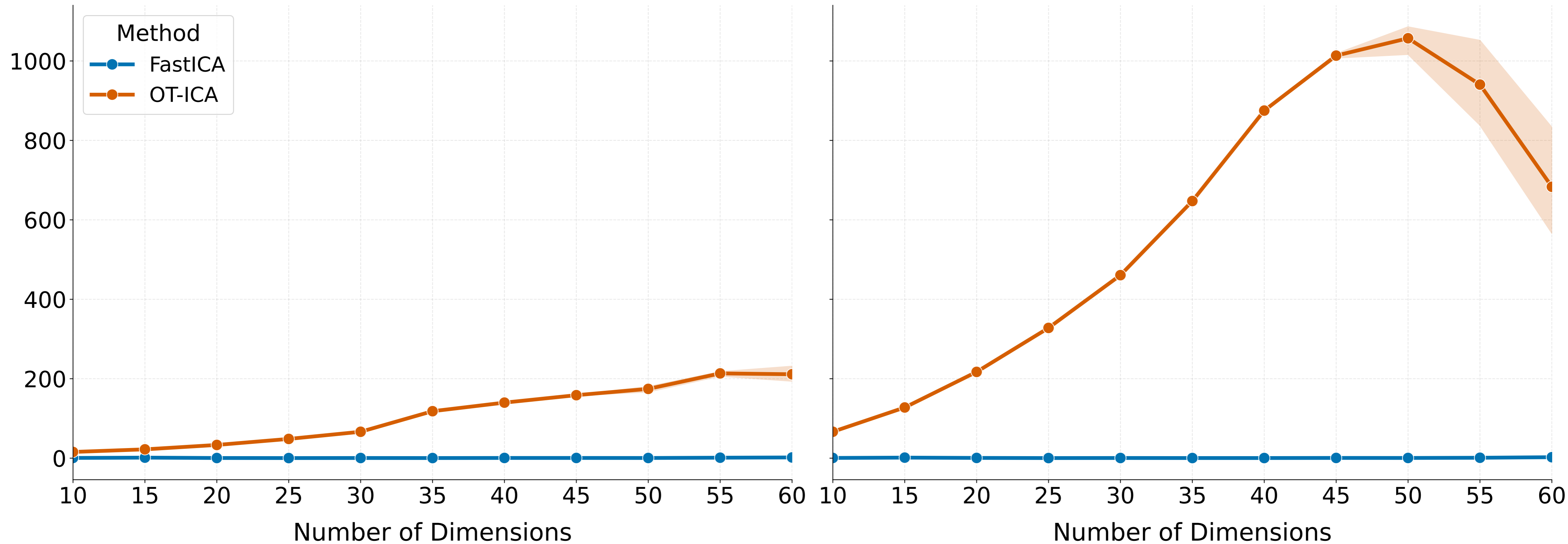
Low Compute Regime
