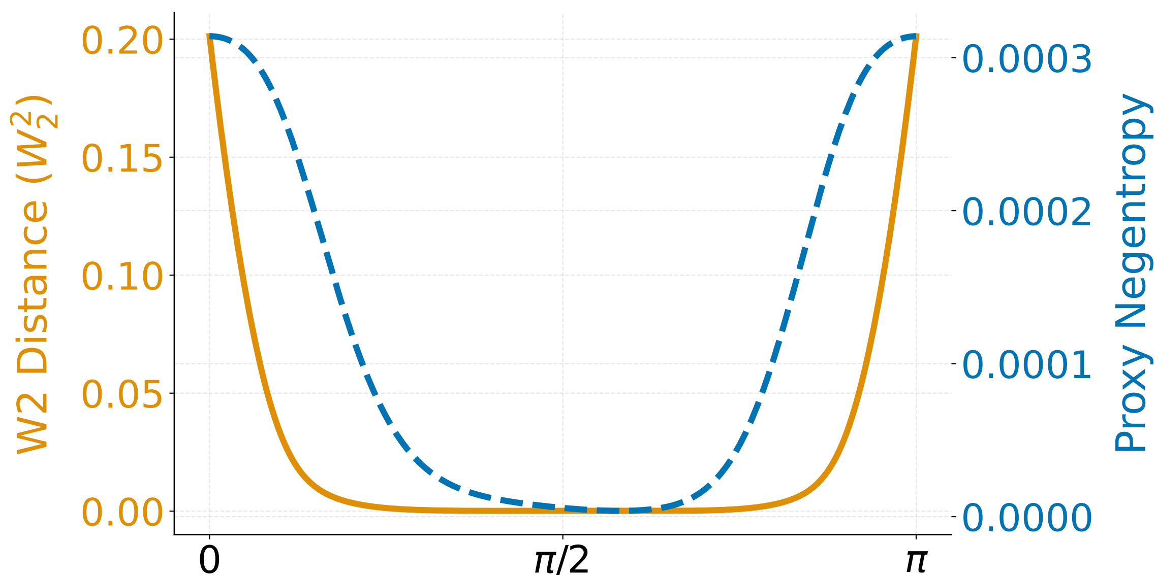
Highly Non-Gaussian Binomial
