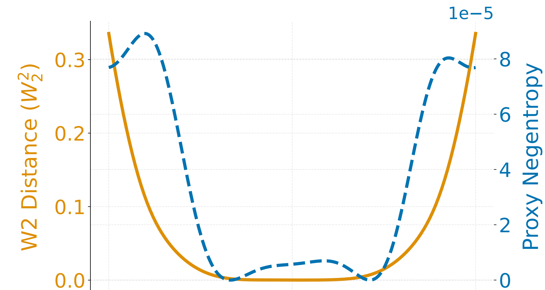
Highly Non-Gaussian Binomial
