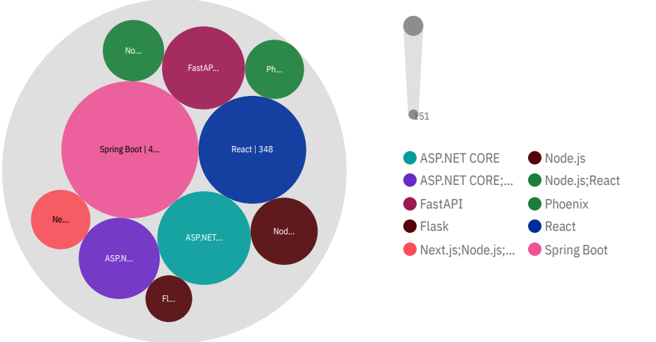
Top 10 WebframeWantToWorkWith
