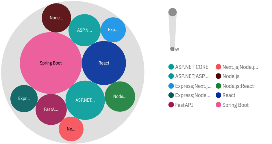
Top 10 WebFrameHaveWorkedWith
