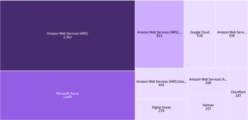
Top 10 PlatformWantToWorkWith
