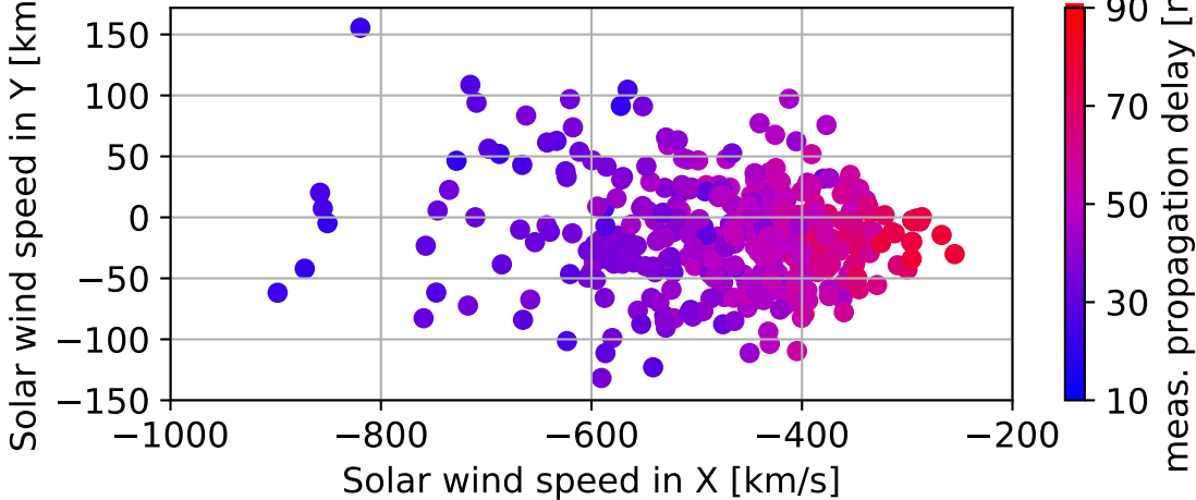
Solar wind speed in GSE
