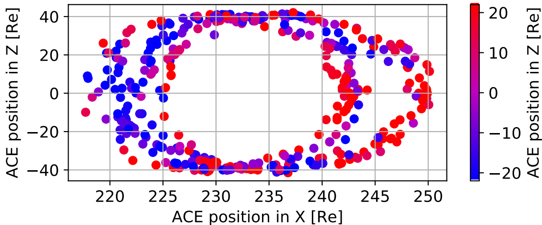
ACE Position in GSE
